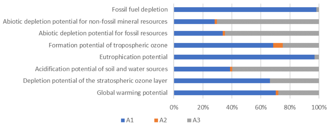
Figure 1. Contribution Analysis: A1-A3 Breakdown Air Entrainers
