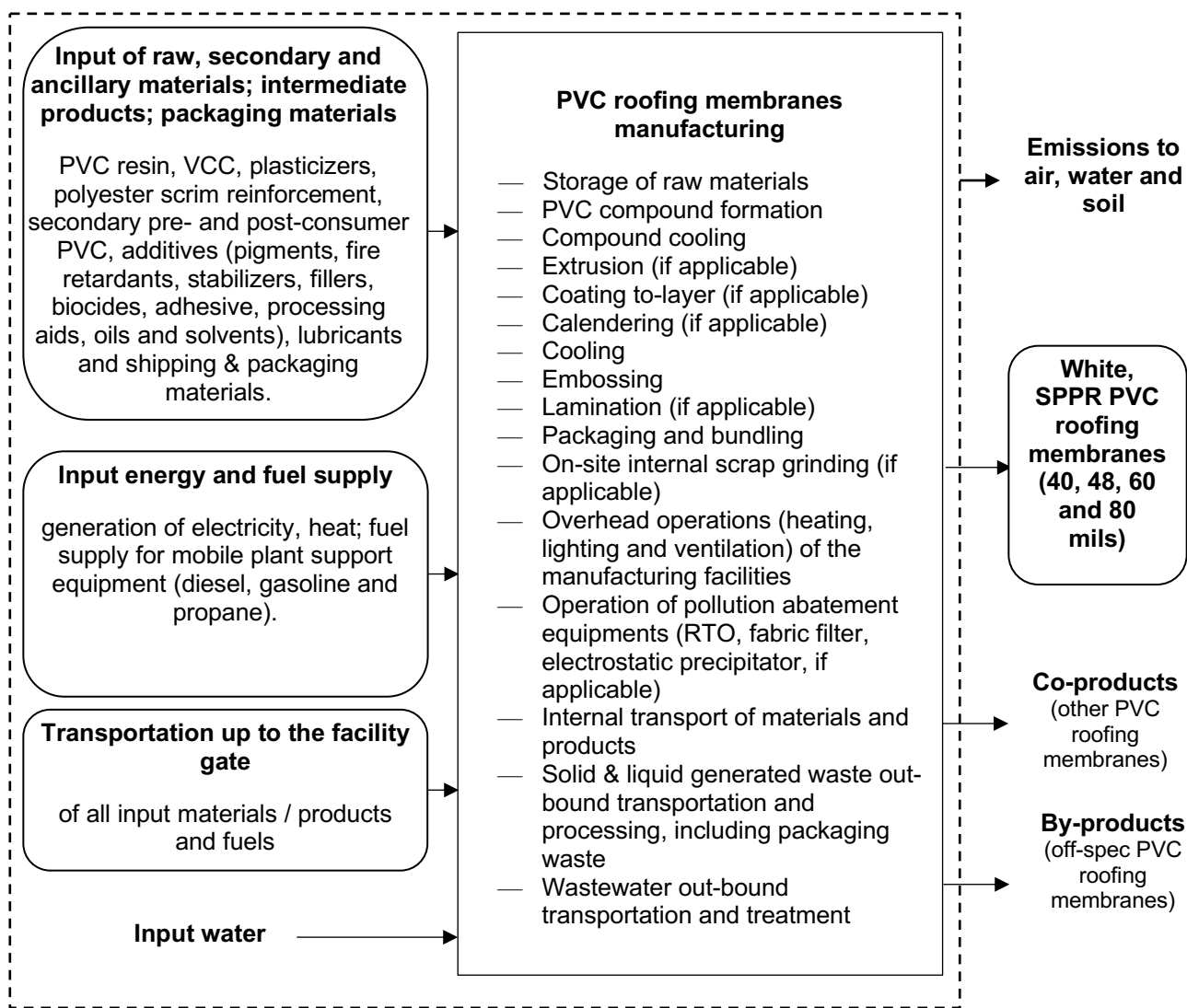
Figure 3 Production stage (module A1 to A3) system boundary of PVC roofing membranes manufacturing
