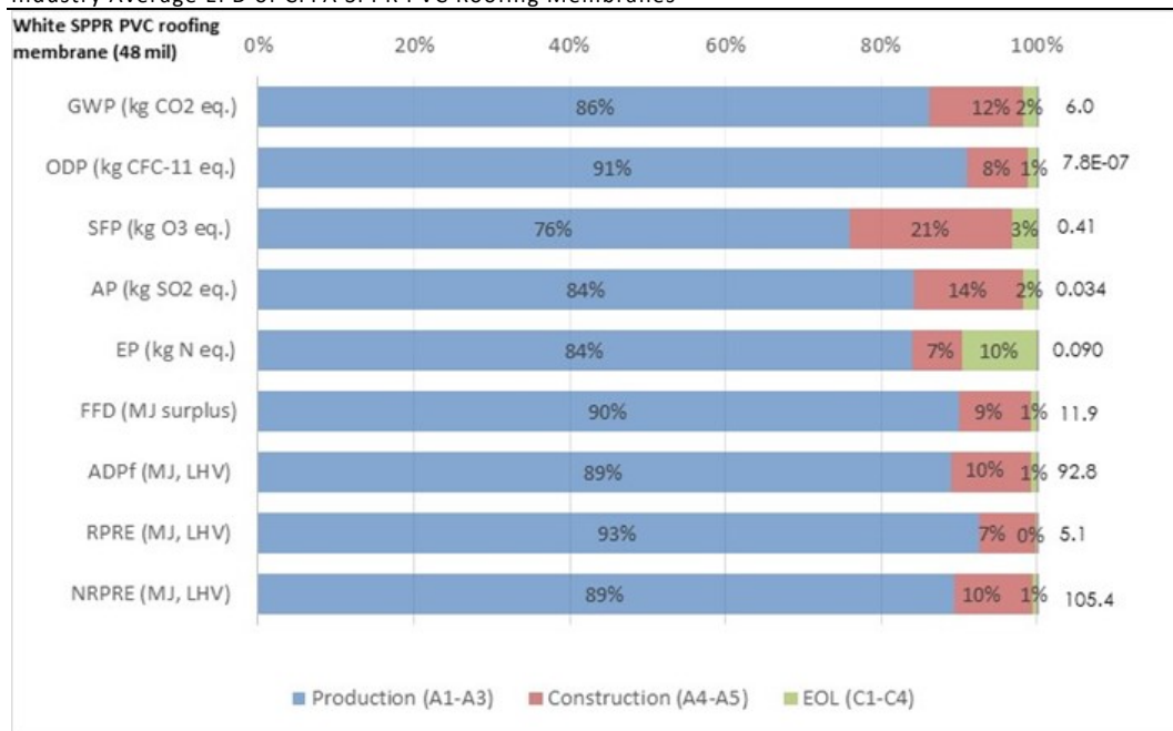
Figure 5 Impact assessment and energy indicator results by stage – 1 m 2 of 48 mils white SPPR PVC roofing membrane – % Basis
