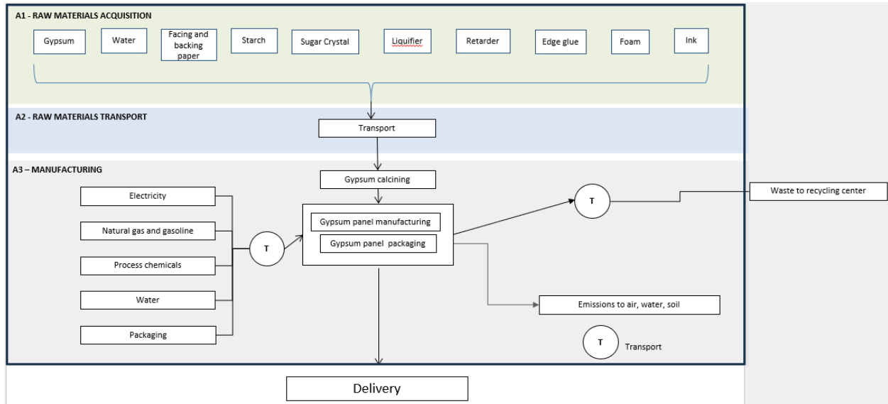
Figure 2: Flow diagram for the Knauf Regular Gypsum Board manufacturing process.
