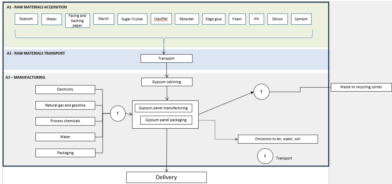
Figure 2: Flow diagram for the Knauf Moisture-Resistant Gypsum Board manufacturing process.
