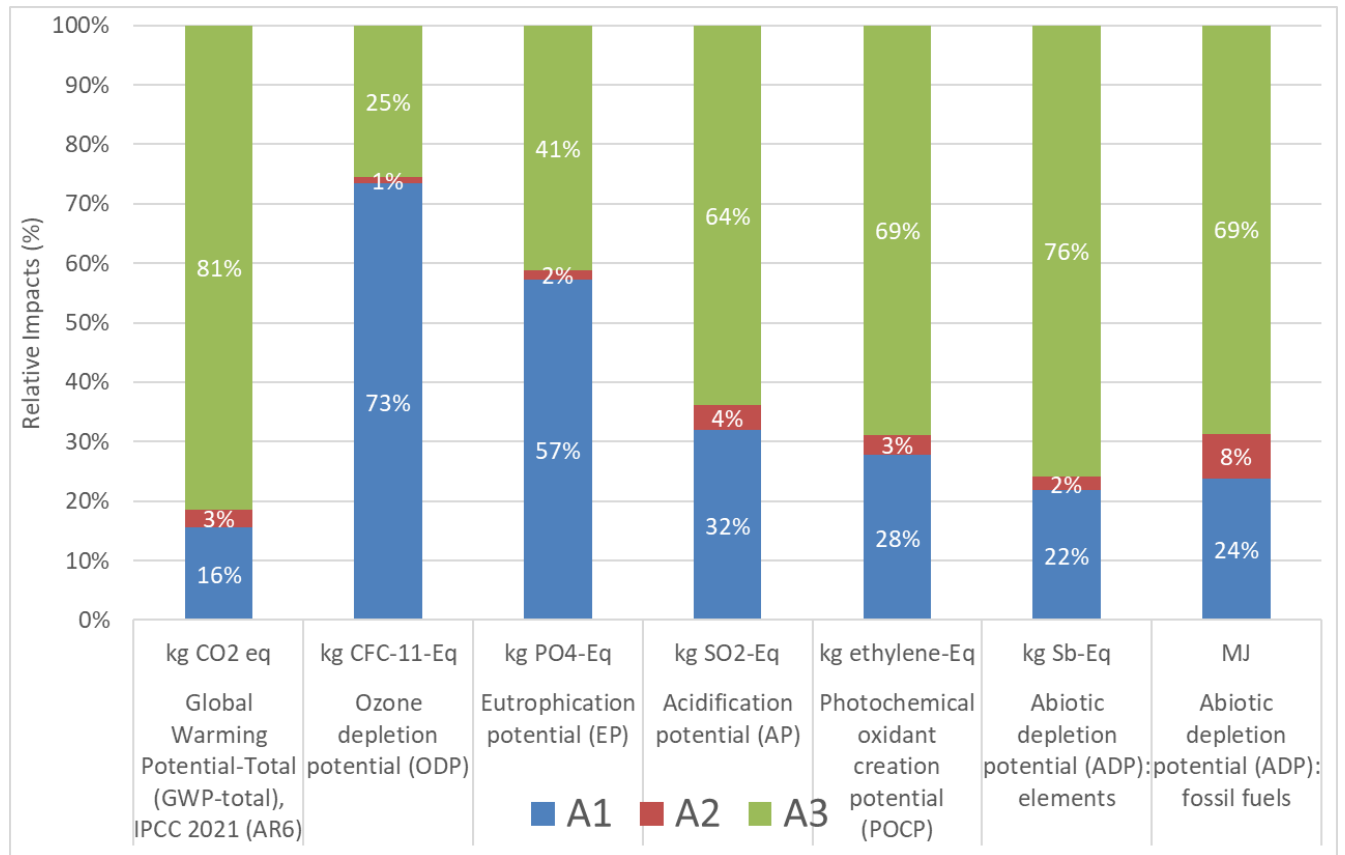
Figure 4: Contribution of each life cycle stage of Moisture-Resistant Gypsum Board
