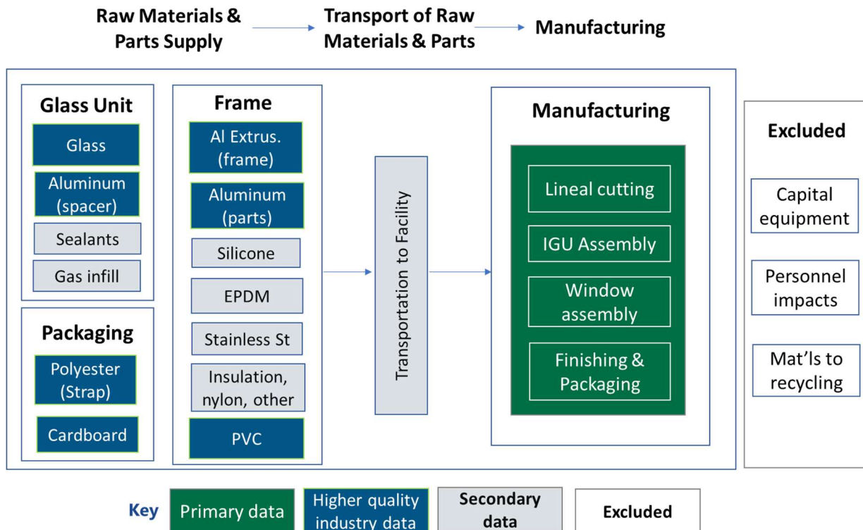
Figure 1 EFCO Storefront System Boundary and Data
