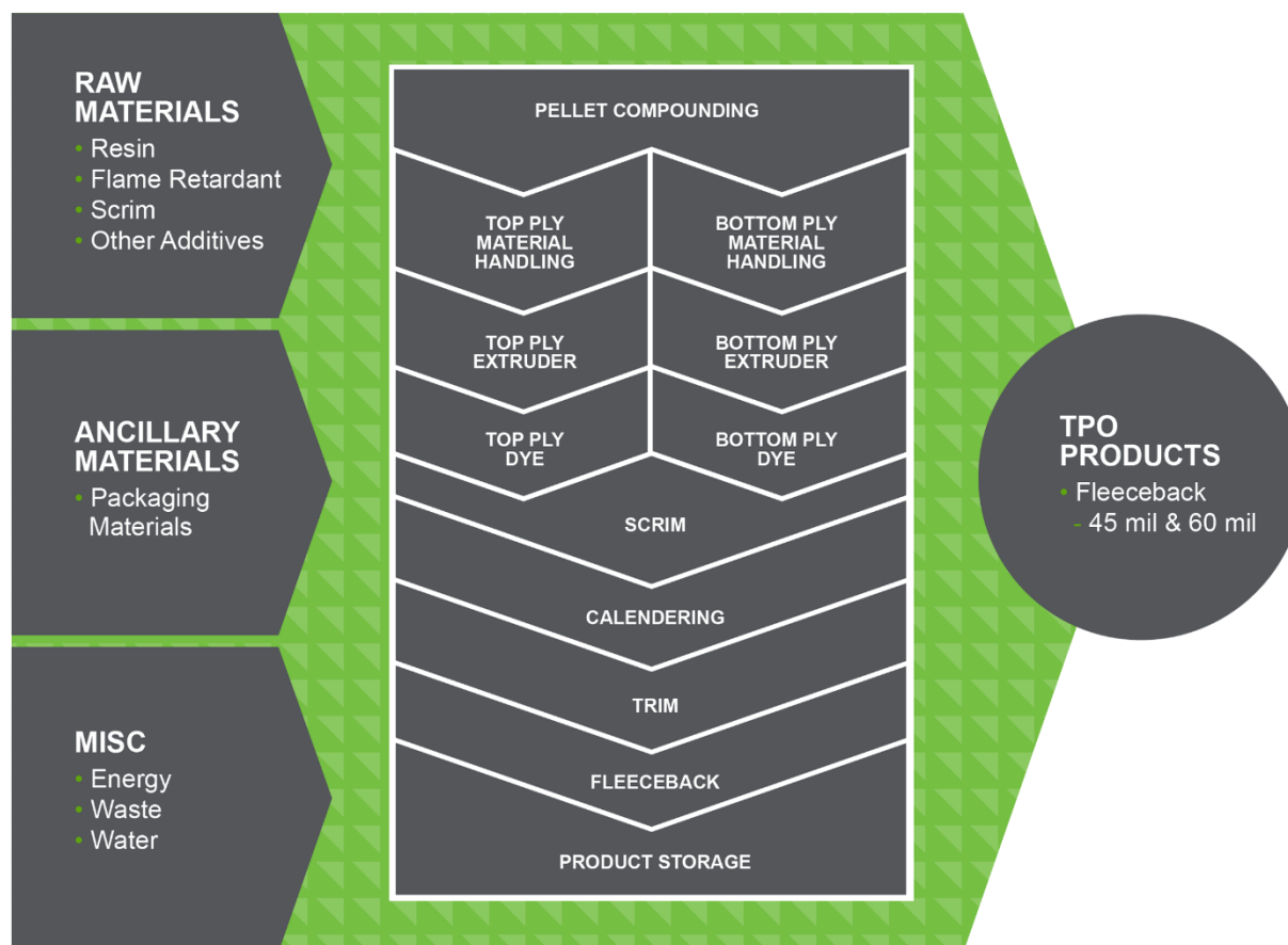
FIGURE 2 Process Flow Diagram of TPO Manufacturing
