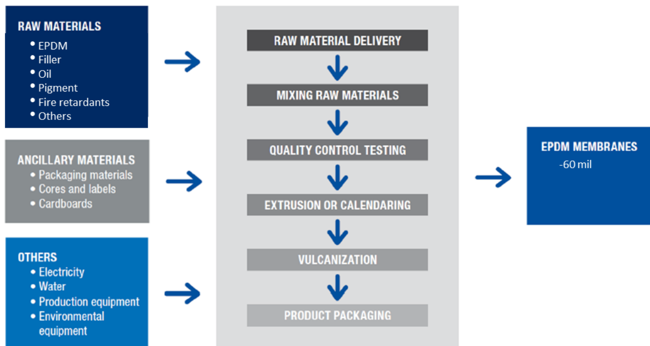
Figure 1: Sure-White® Reinforced EPDM production process map
