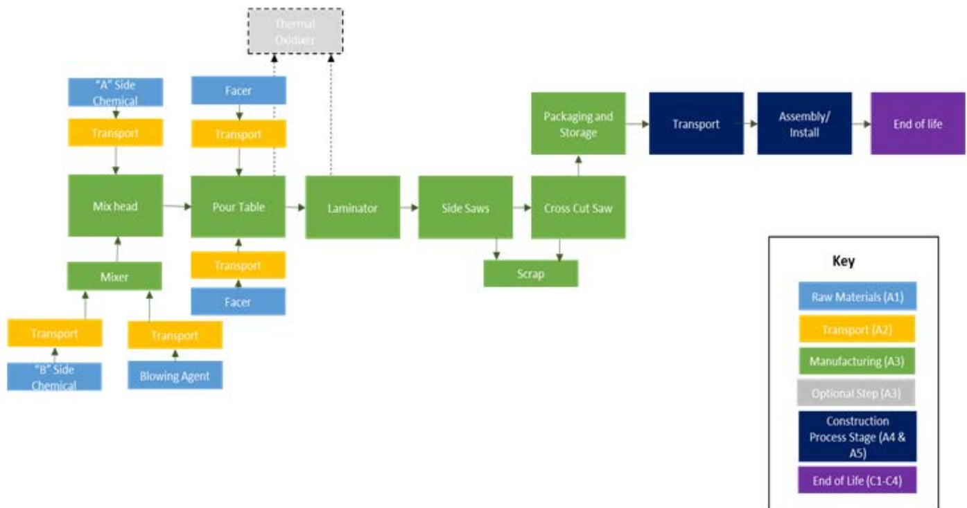
Figure 4: Process Flow Diagram for Polyiso Roof Insulation Boards.
