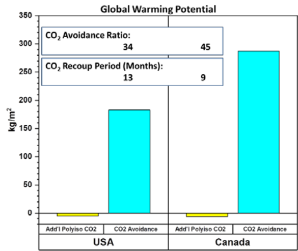
Figure 8: National average results for Global Warming Potential
