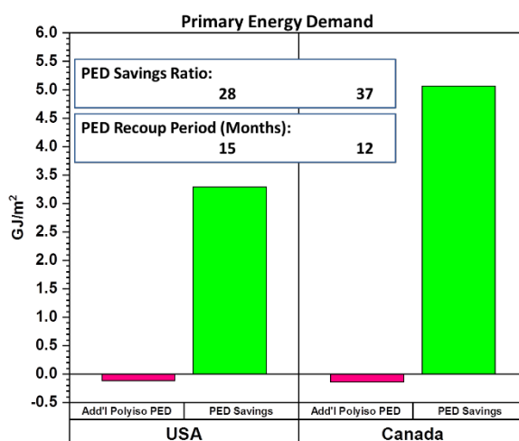
Figure 7: National average results for Primary Energy Demand
