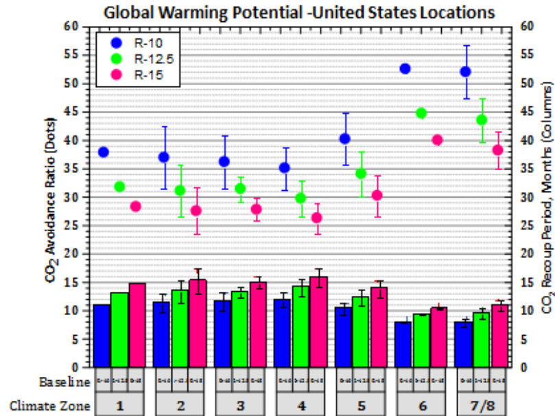
Figure 9: U.S. location results for Global Warming Potential
