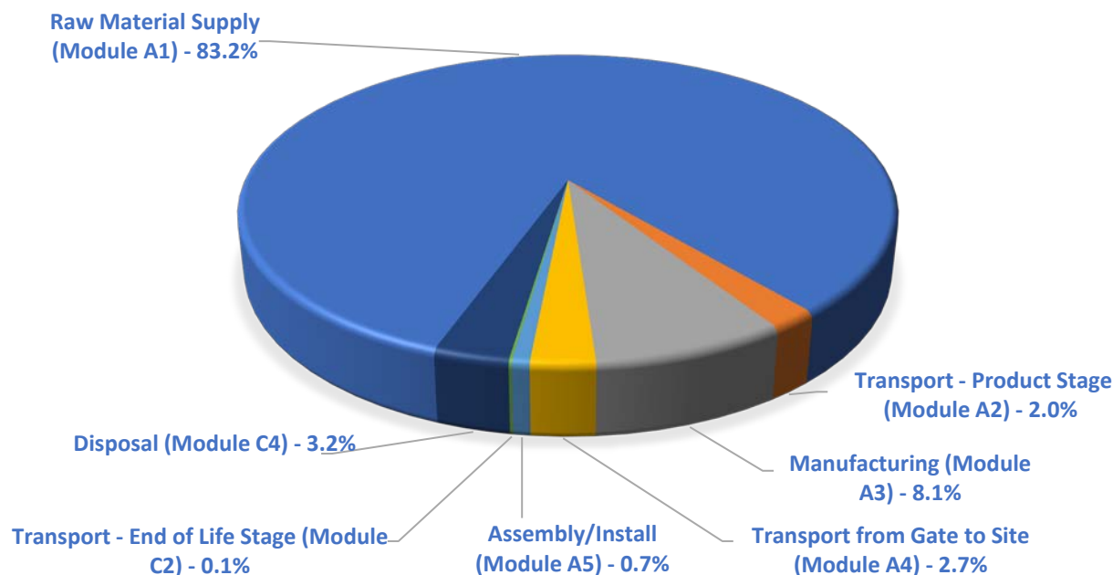
Figure 6: Relative Impact of Modules on Global Warming Potential for CGF Faced Polyiso Roof Insulation Boards.
