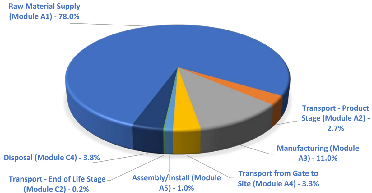
Figure 5: Relative Impact of Modules on Global Warming Potential for GRF Faced Polyiso Roof Insulation Boards.
