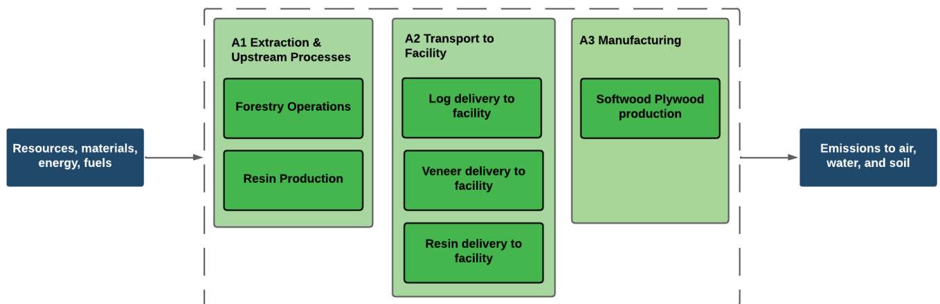
Figure 3. Cradle-to-Gate (A1-A3) System Boundary for Southern Softwood Plywood Production.
