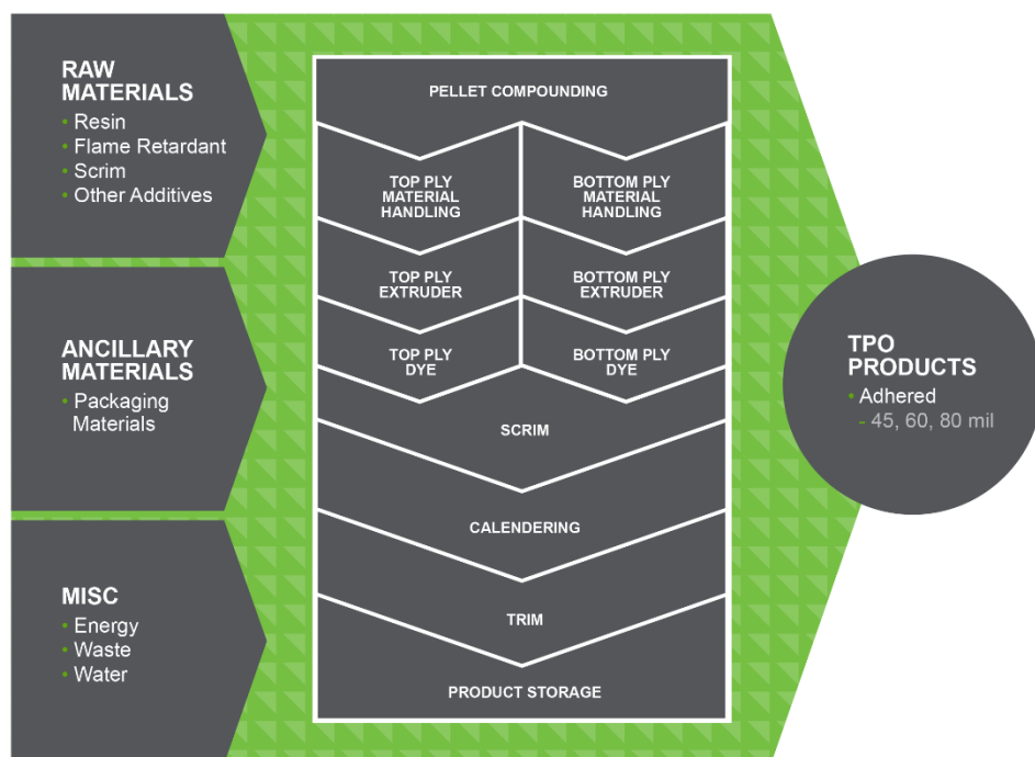
FIGURE 2 Process Flow Diagram of TPO Manufacturing
