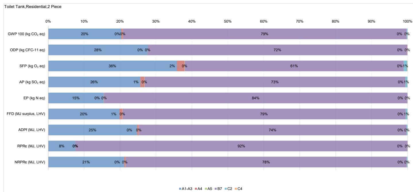
Figure 3. Cradle-to-grave (A1-C4) EPD results –Residential 2-piece toilet tank product group (weighted average)- % Contribution by module
