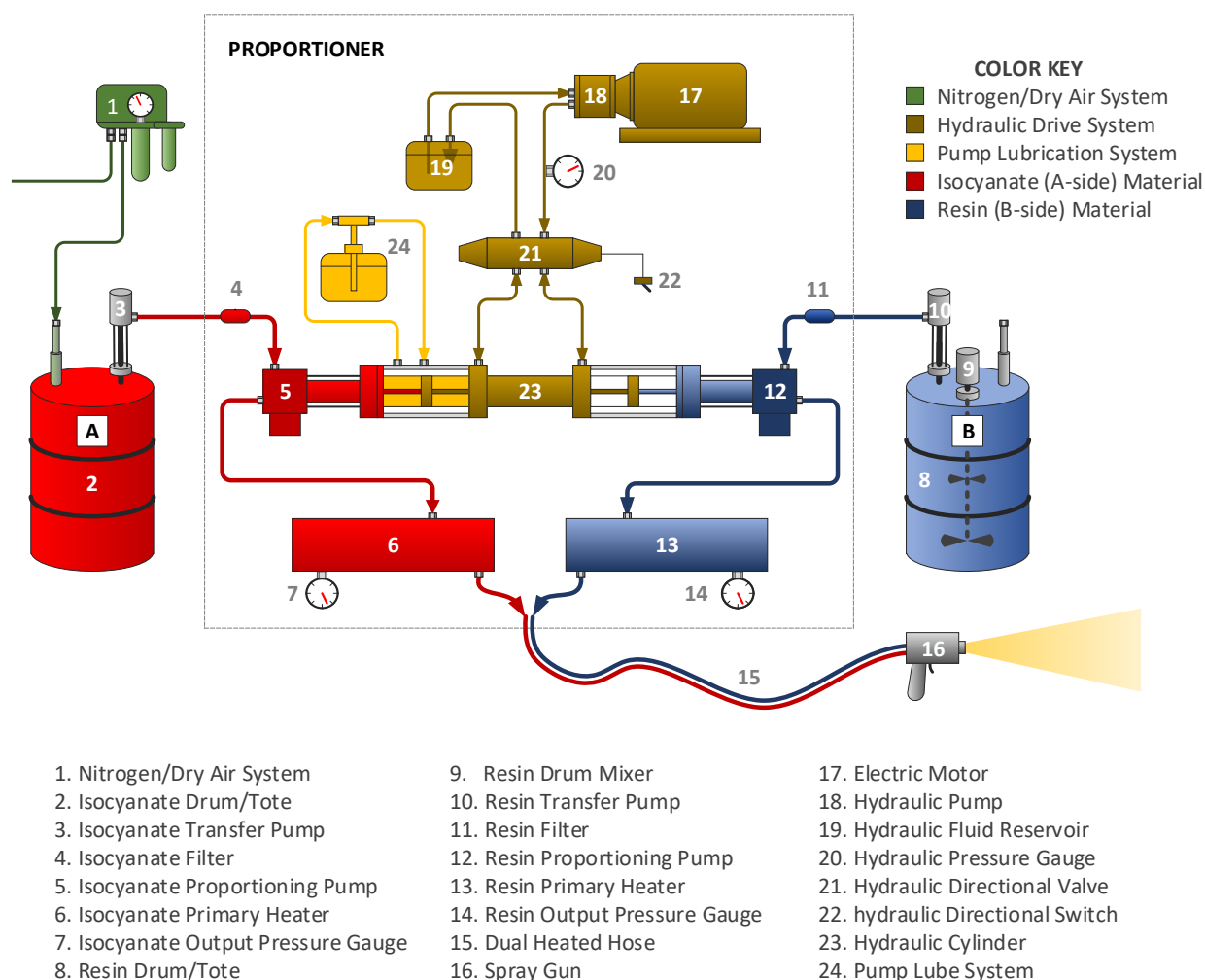
Figure 3. Schematic of a High-Pressure SPF system
