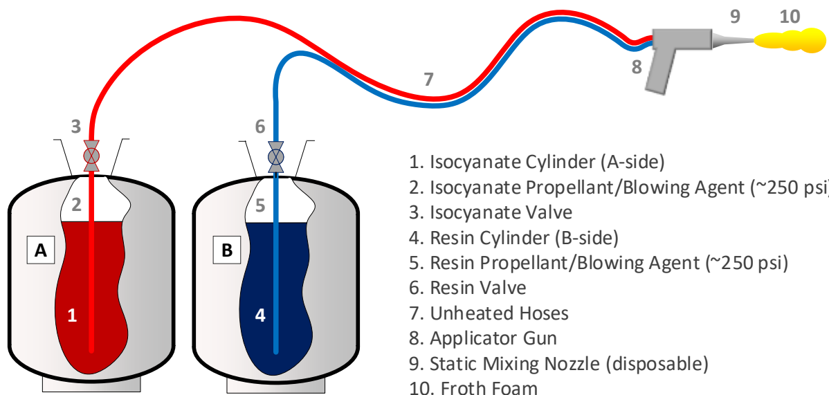
Figure 4. Schematic of a Low-Pressure SPF system
