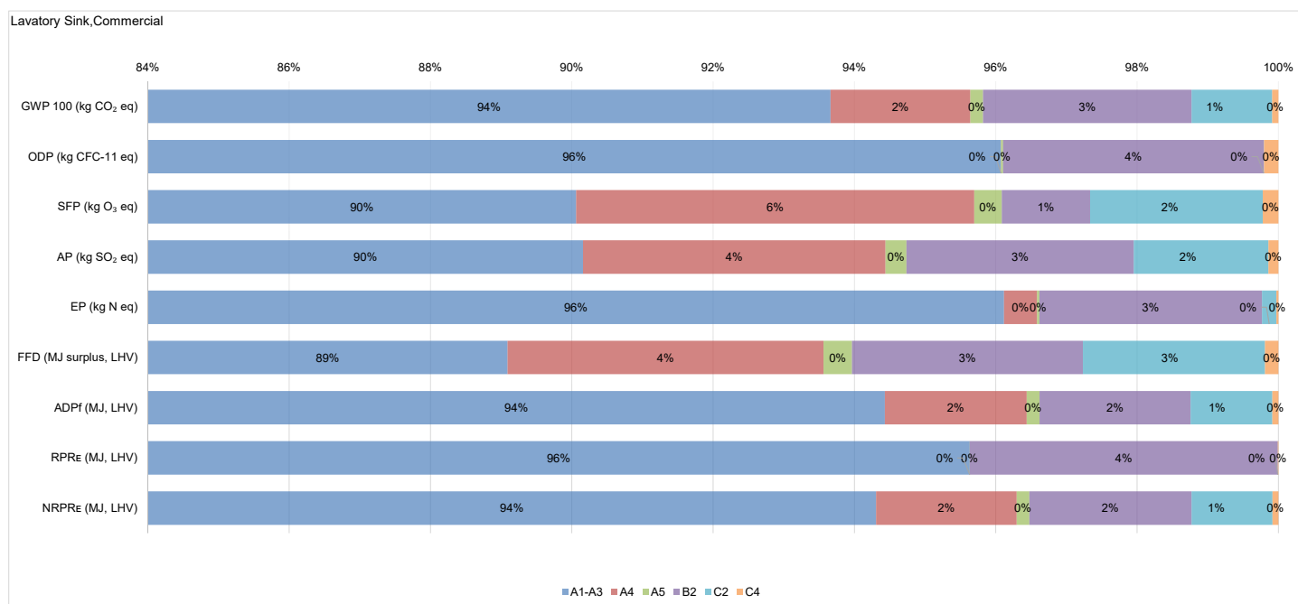
Figure 3. Cradle-to-grave (A1-C4) EPD results – Commercial lavatory sink product group (weighted average)- % Contribution by module
