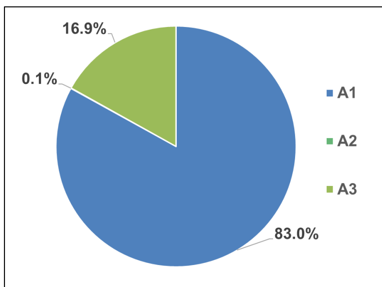
Figure 3: Process Dominance Analysis for GWP for the Production of 1 Tonne of Red Top® Keenes Cement (A1-A3) – Shoals, IN Plant
