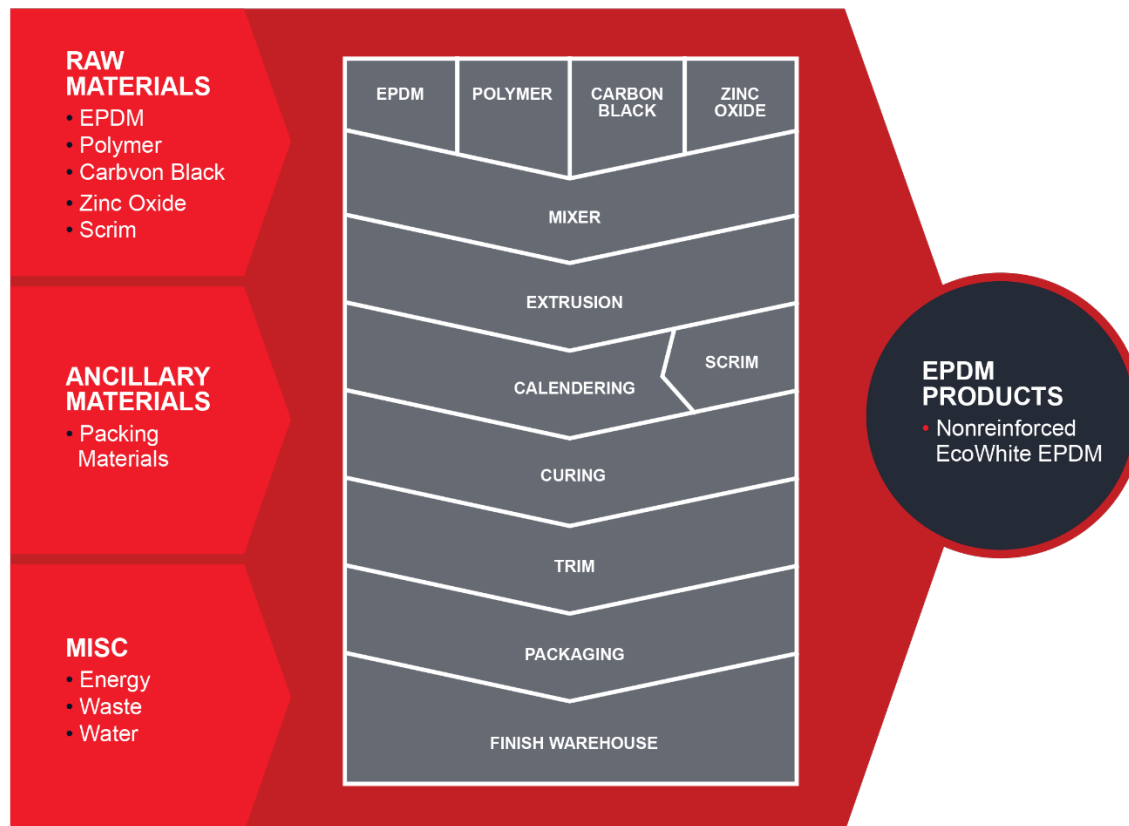
FIGURE 2 Process Flow Diagram of EPDM
