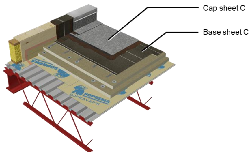
Figure 1. Visual representation of the cold-adhered SBS-modified bitumen membrane
