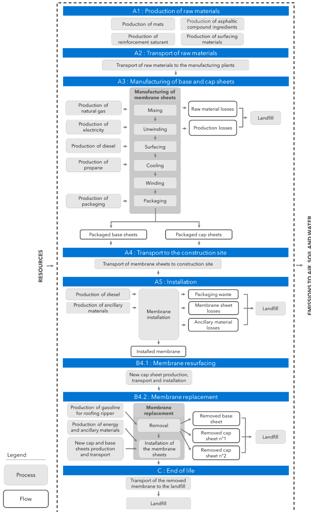
Figure 3: System boundary - SBS-modified bitumen membrane – cold-adhered
