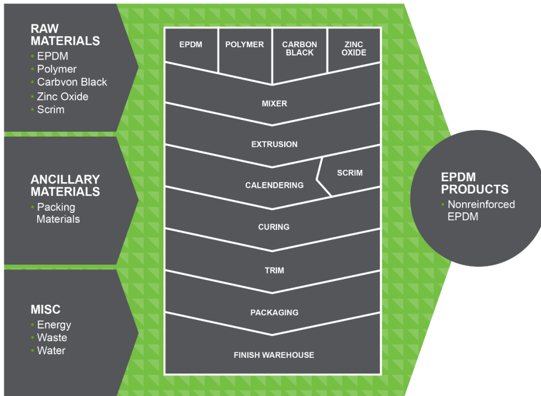
FIGURE 2 Process Flow Diagram of EPDM
