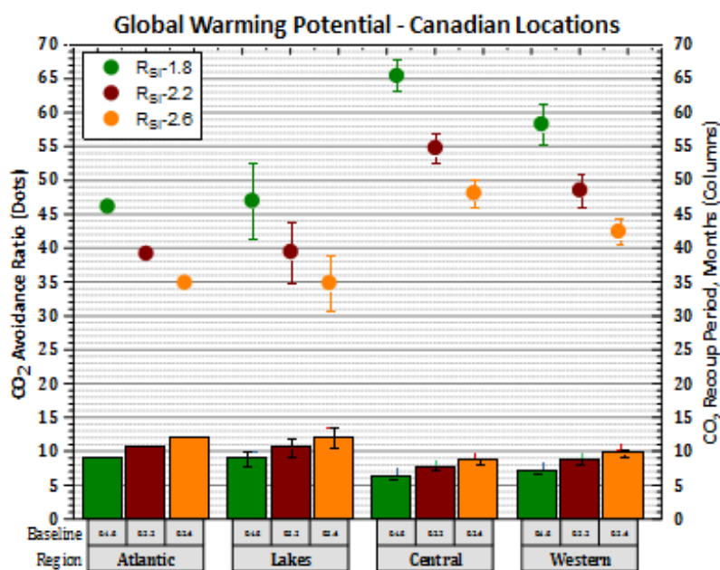
Figure 10: Canada location results for Global Warming Potential
