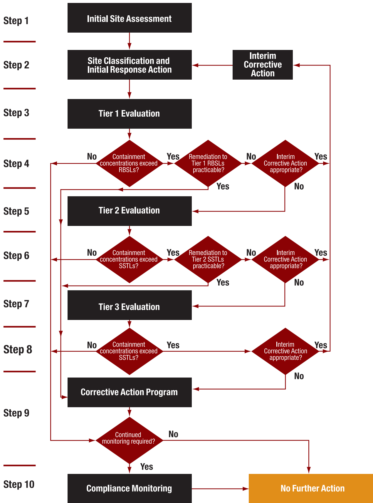
ASTM Risk-Based Corrective Action (RBCA) Flowchart
